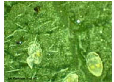
Whitefly nymphs
